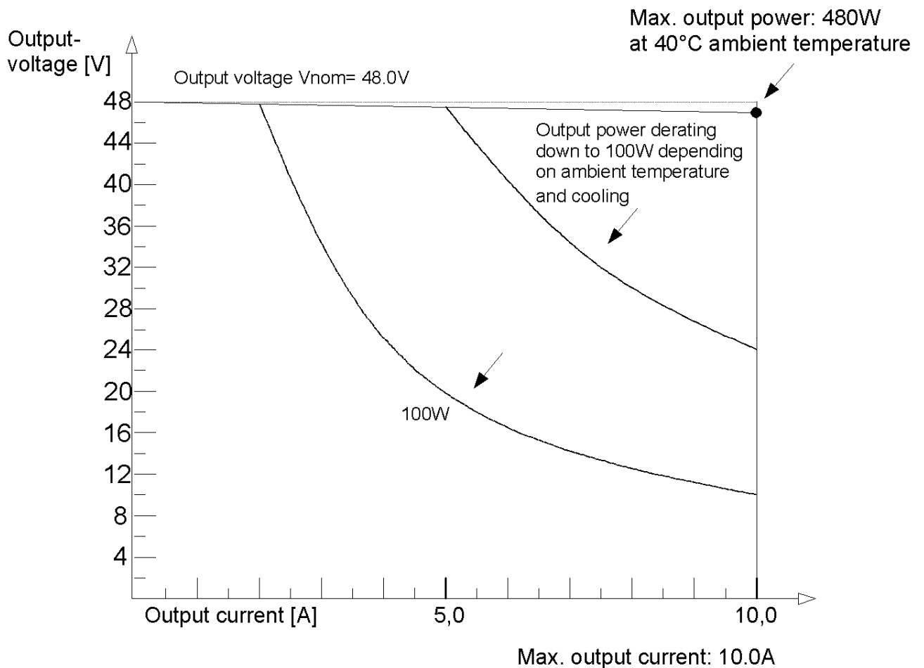
Figure 6.) Output power diagram
